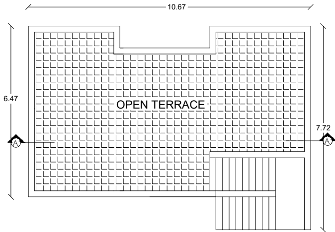
TERRACE FLOOR
