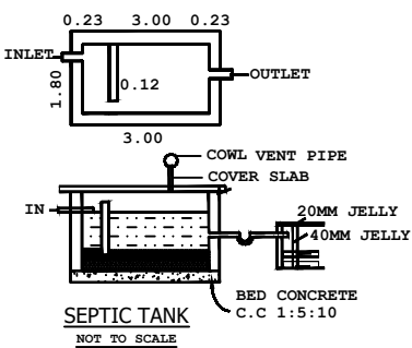
SEPTIC TANK NOT TO SCALE
