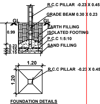
FOUNDATION DETAILS
