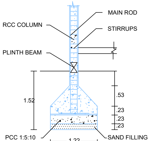
COLUMN DETAILS
