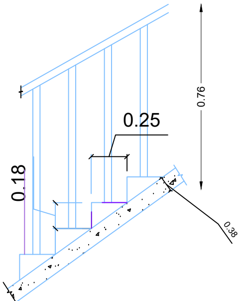
SECTION OF STAIRCASE
