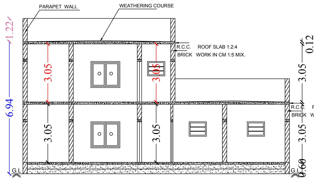
Section on-"AA"
