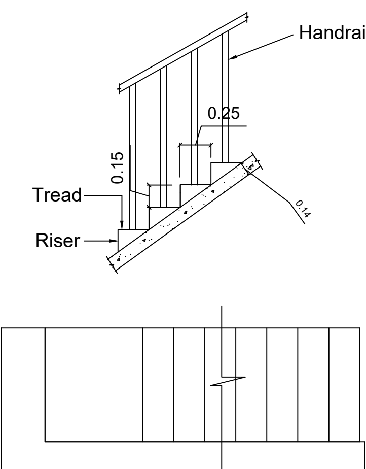
STAIRCASE DETAIL
