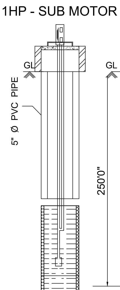
BOREWELL DETAILS
