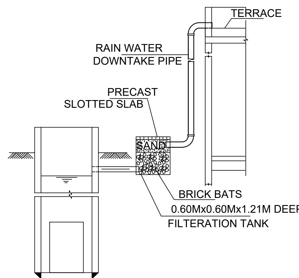
RAIN WATER HARVESTING SYSTEM
