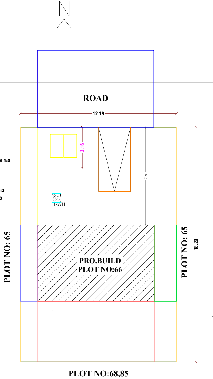
SITE PLAN
