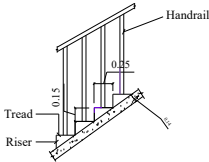
STAIRCASE DETAIL
