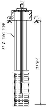
BOREWELL DETAILS
