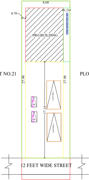
Site Plan
