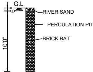
PERCOLATION PIT
