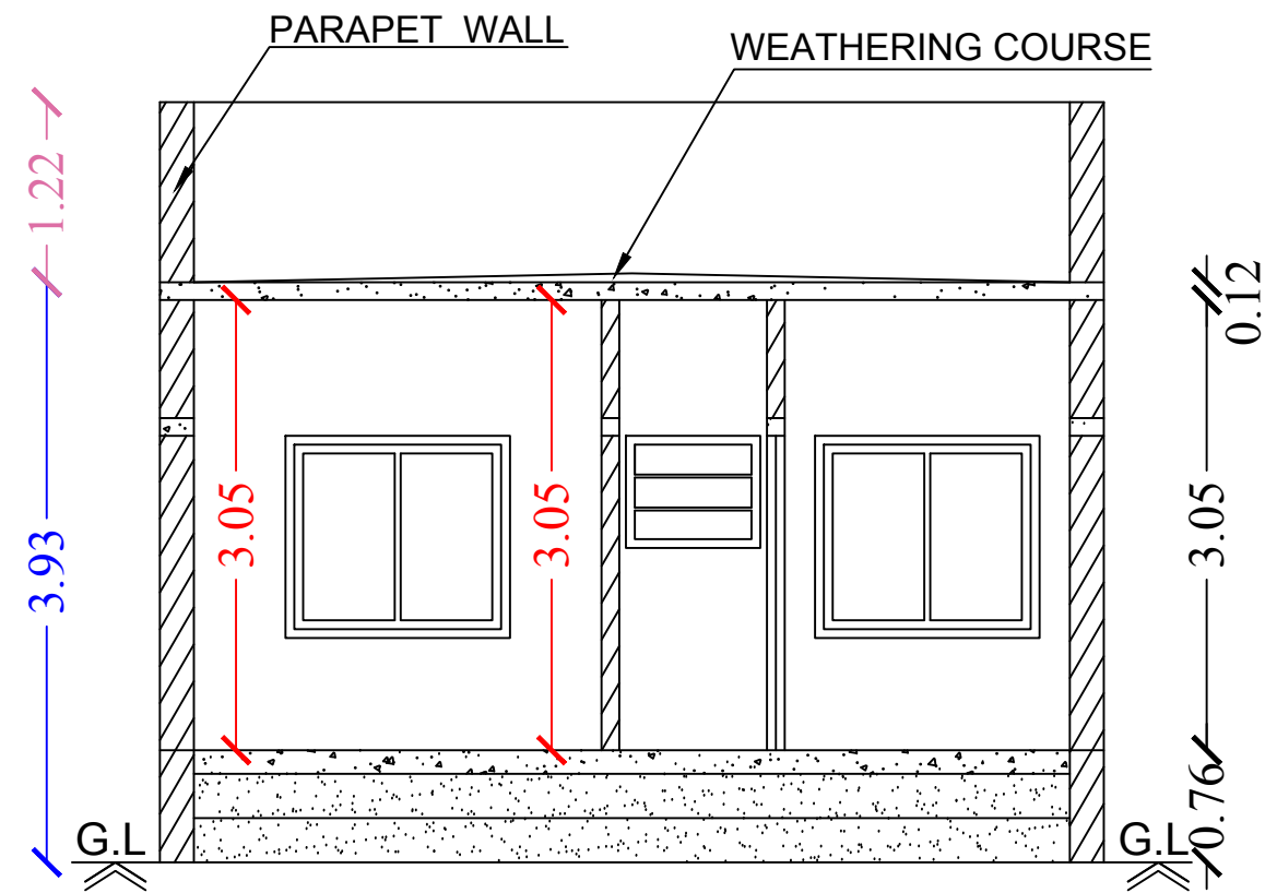
Section on-"AA"
