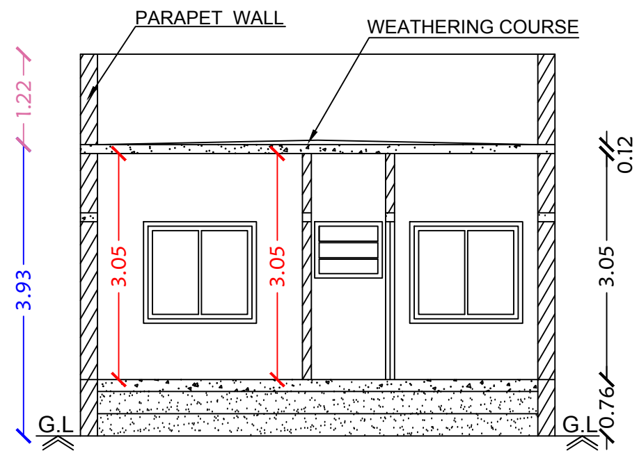
Section on-"AA"
