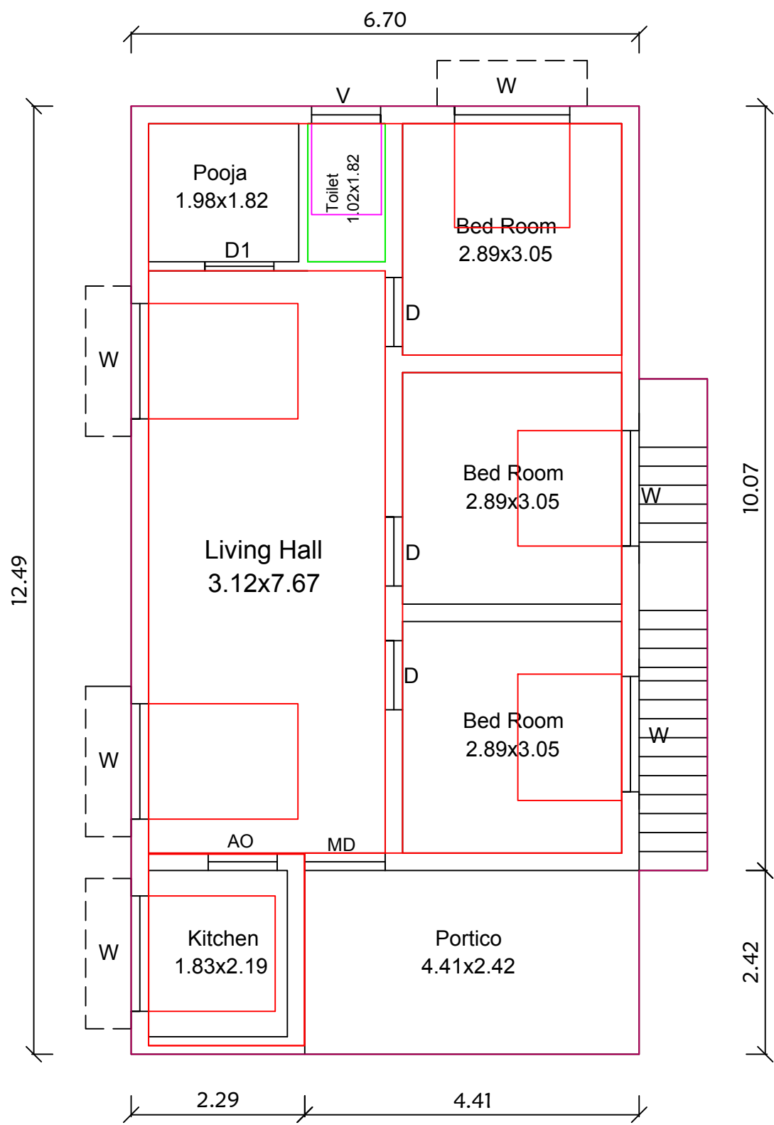
Ground Floor
