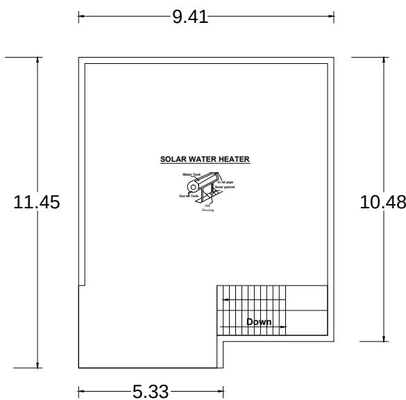
Open Terrace Plan
