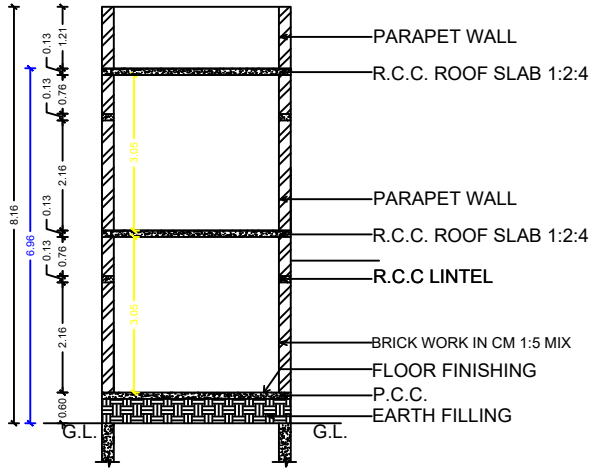
SECTION ON "VR"
