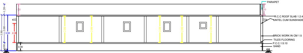
SECTION ON A-B
