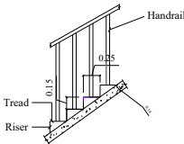
STAIRCASE DETAIL
