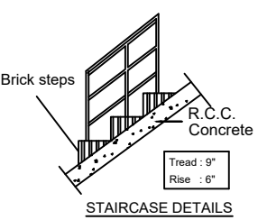
STAIRCASE DETAILS
