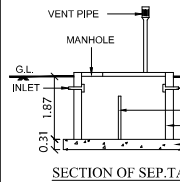
SECTION OF SEPTIC TANK
