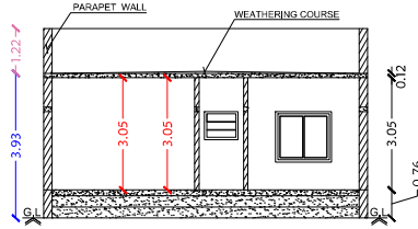
Section on-"AA"
