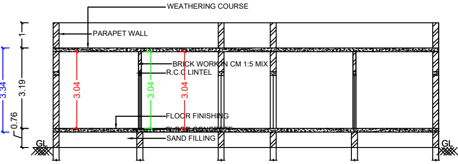
SECTION AT A1-A1
