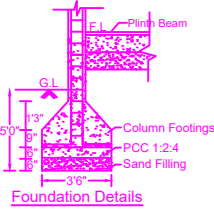
Foundation Details
