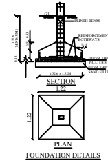
FOUNDATION DETAILS
