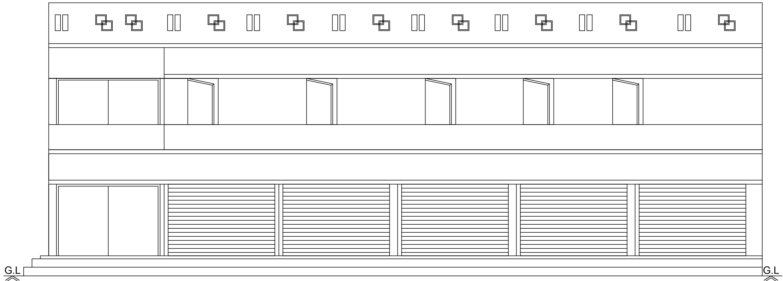
Front Elevation
