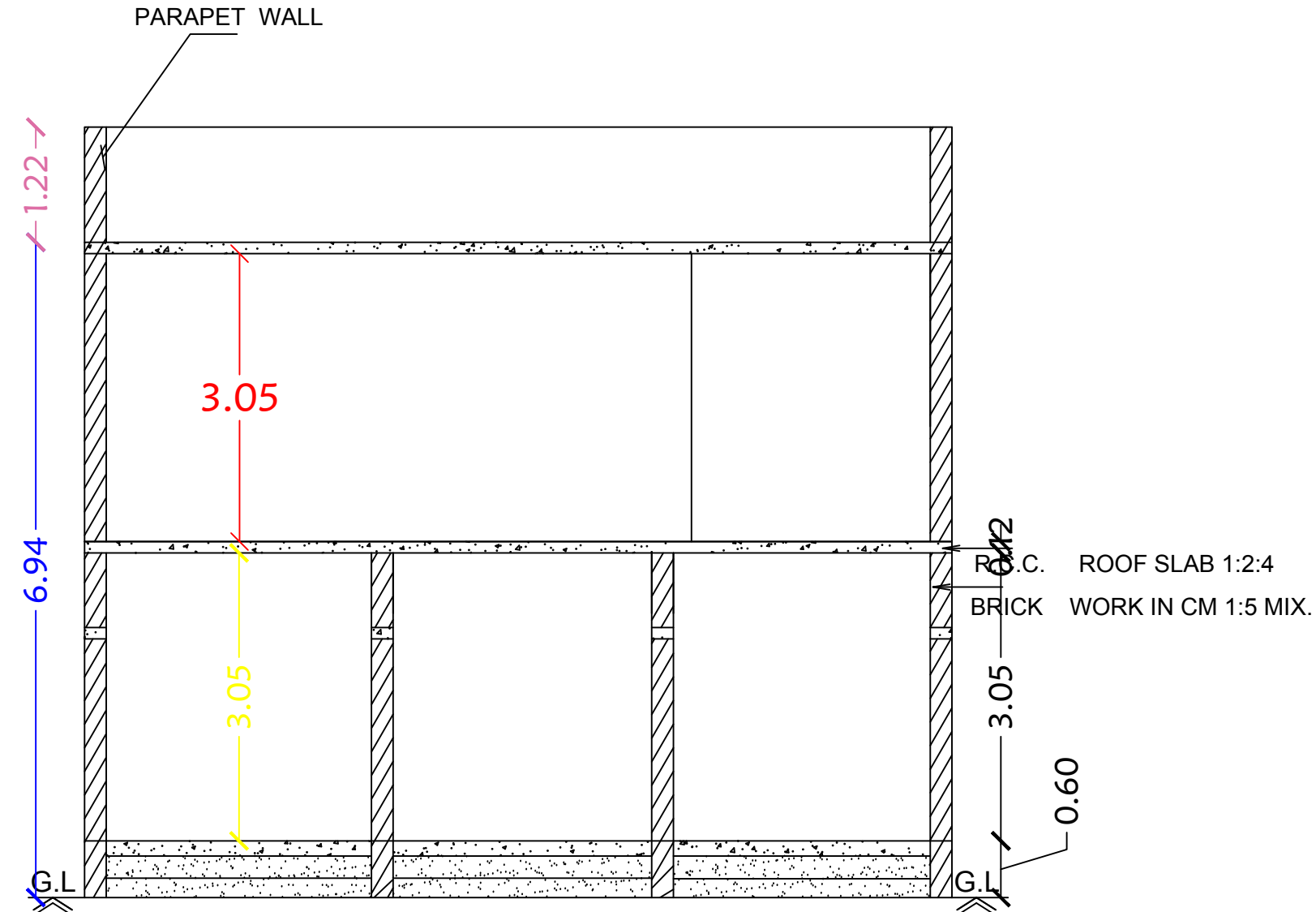
Section on-"AA"
