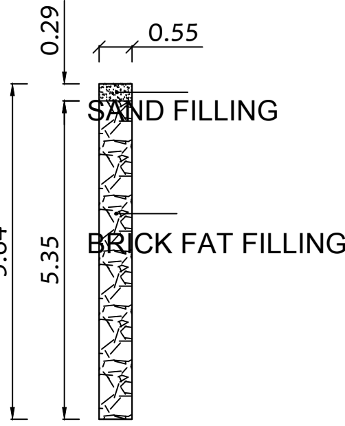
DETAILS OF PERCULATION PIT
