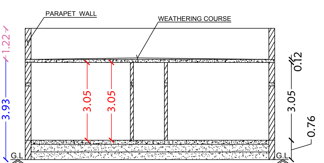
Section on-"AA"
