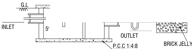
SECTION-AB
