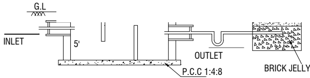
SECTION-AB
