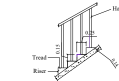
STAIRCASE DETAIL
