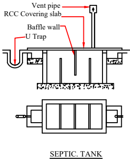
SEPTIC TANK
