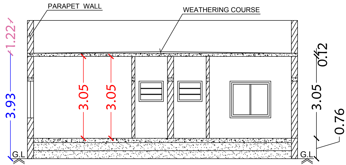
Section on-AA'
