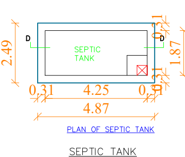
SEPTIC TANK
