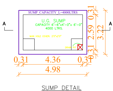
SUMP DETAIL
