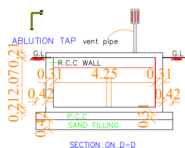
SECTION ON D-D
