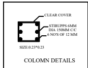
COLUMN DETAILS
