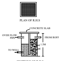
SECTIONS OF R.H.S.
