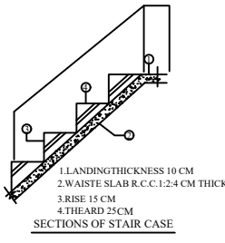
SECTIONS OF STAIR CASE
