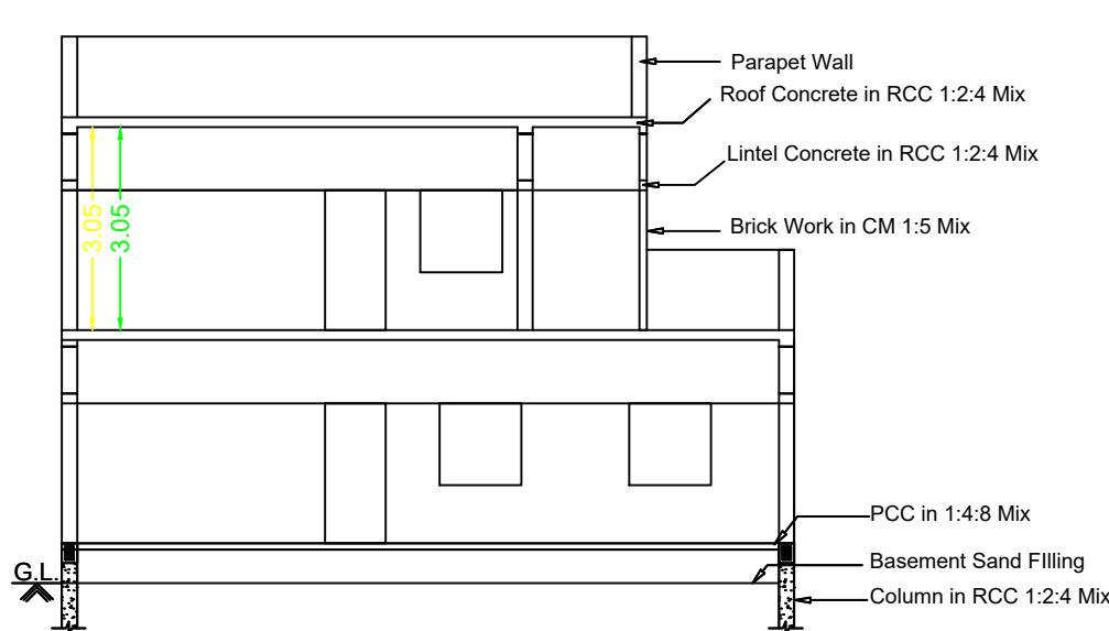
Section RR
