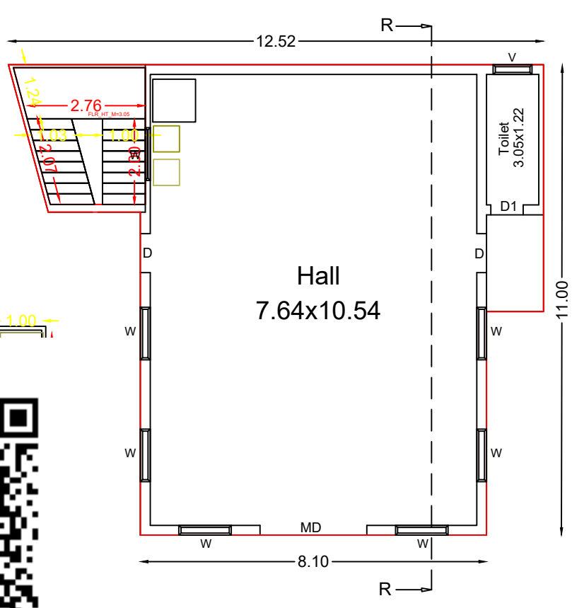
Ex.Ground & Pro.First Floor Plan
