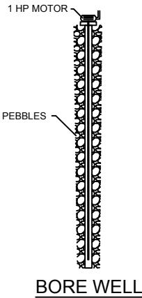
BORE WELL
