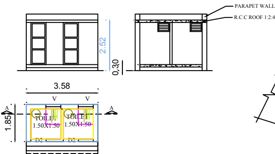
PLAN, SECTION & ELEVATION OF TOILET BLOCK
