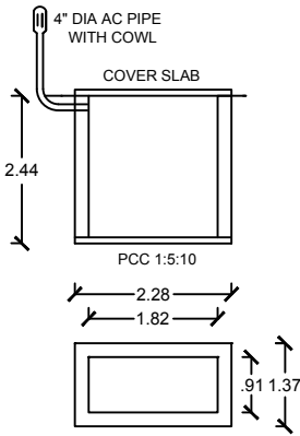
SEPTIC TANK
