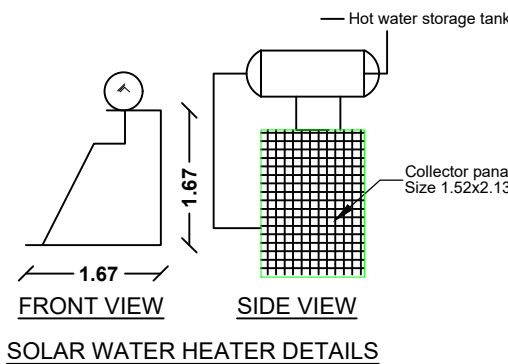
SOLAR WATER HEATER DETAILS
