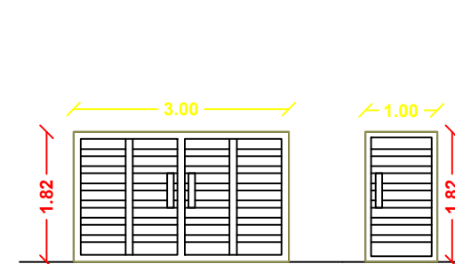
MAIN GATE
