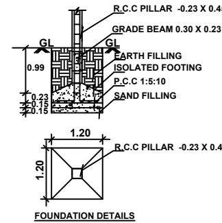
FOUNDATION DETAILS
