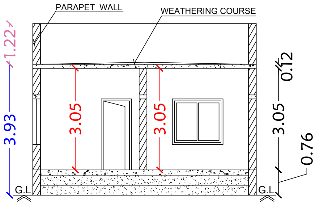
Section on-"AA"
