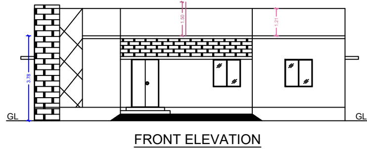
FRONT ELEVATION
