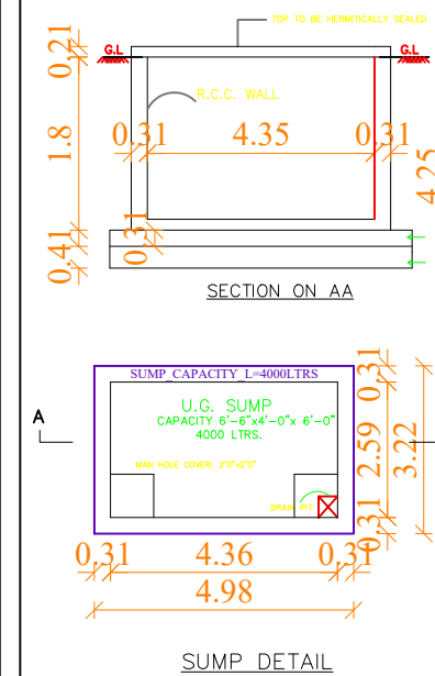
SUMP DETAIL
