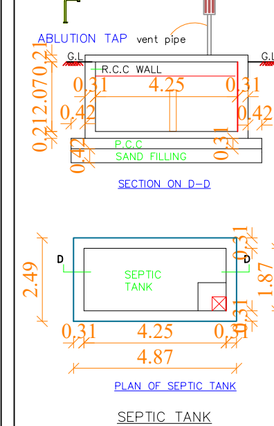
SEPTIC TANK
