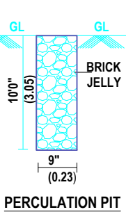
PERCOLATION PIT
