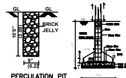
PERCOLATION PIT
