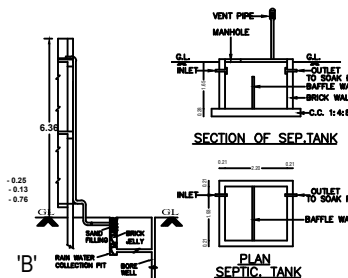
RAIN WATER HARVESTING SYSTEM RW_H_CAPACITY_L=1000LTRS
