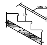
STAIR CASE DETAILS
