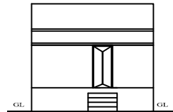
FRONT ELEVATION
