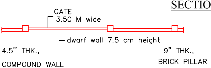
COMPOUND WALL PLAN
