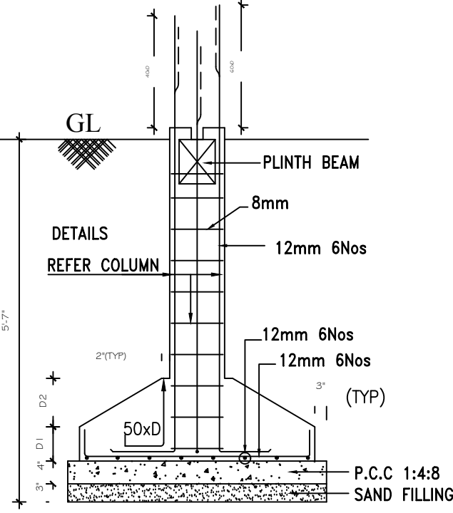
FOUNDATION DETAILS
