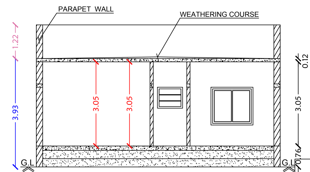
Section on-"AA"
