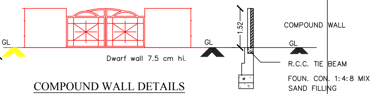
COMPOUND WALL DETAILS
