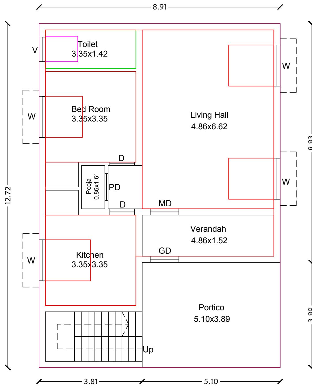
Ground Floor
