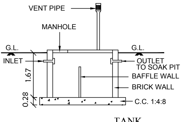
TANK
