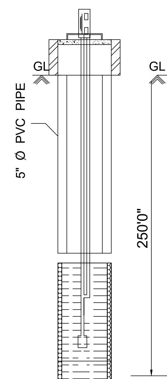
BOREWELL DETAILS
