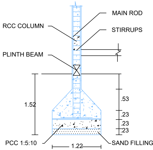
COLUMN DETAILS
