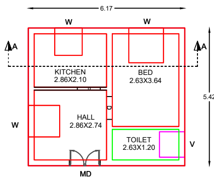
PROPOSED RESIDENTIAL GROUND FLOOR PLAN
