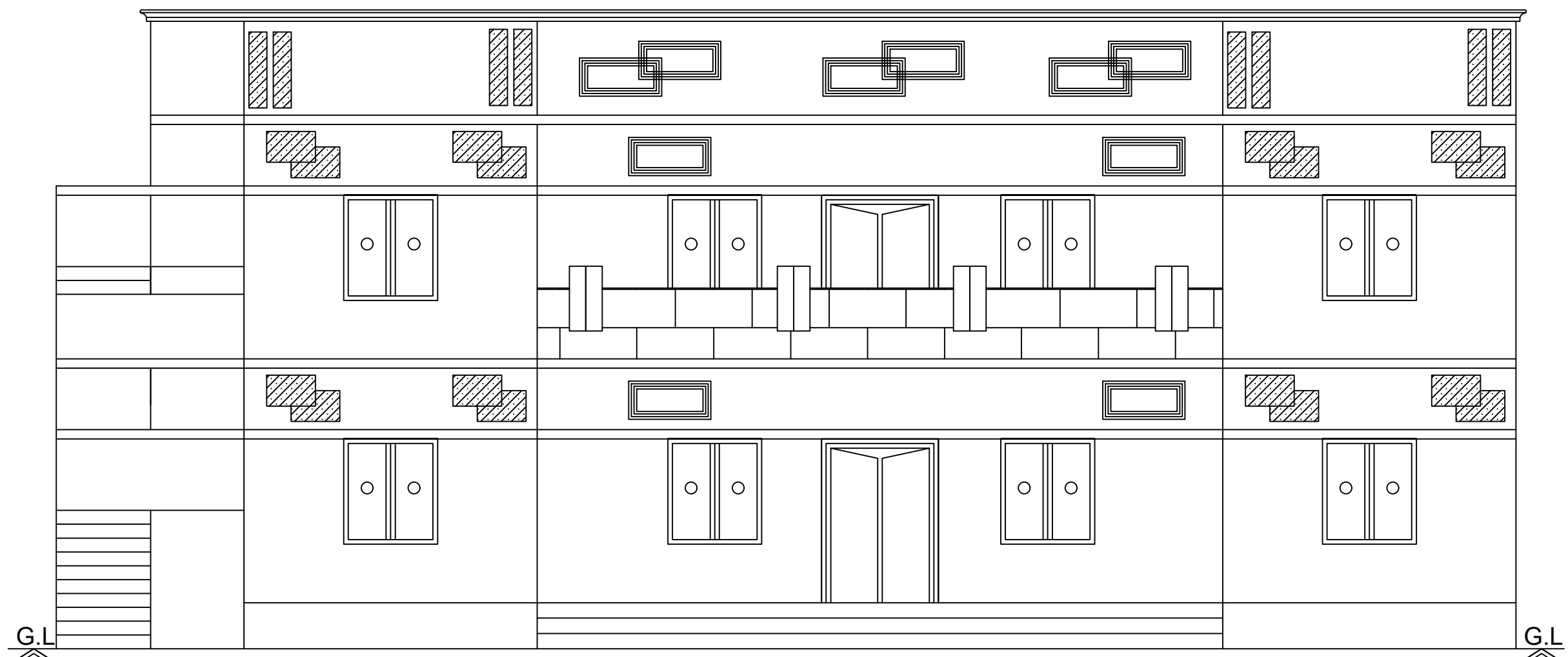
Front Elevation
