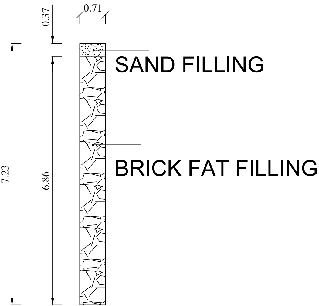
DETAILS OF PERCULATION PIT
