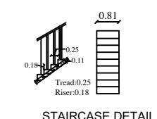
STAIRCASE DETAIL
