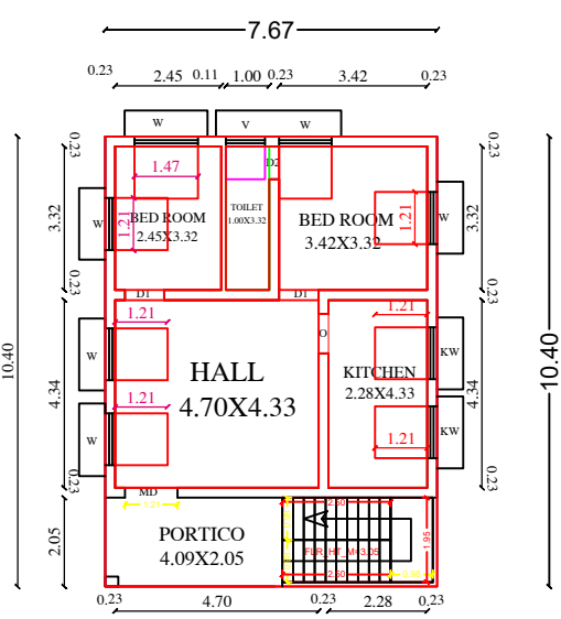
PRO.G.FLOOR.PLAN
