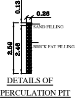
SECTION
