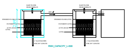
RAIN WATER HARVESTING SYSTEM
