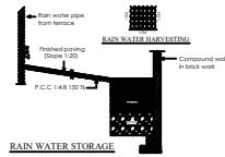
RAIN WATER STORAGE
