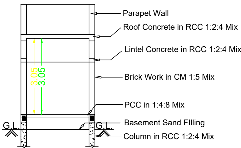
Section RR
