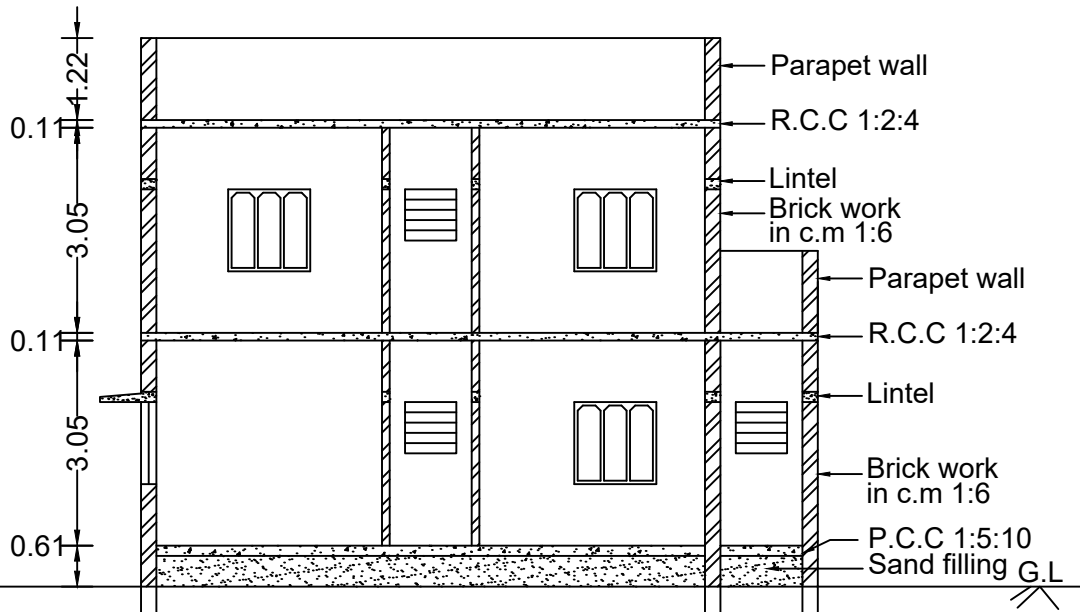
CROSS SECTION ON"AB"
