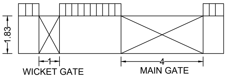
COMPOUND WALL
