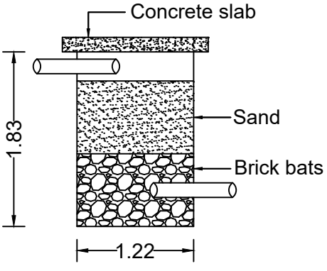
RAIN WATER STORAGE
