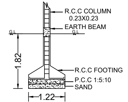
FOUNDATION DETAILS
