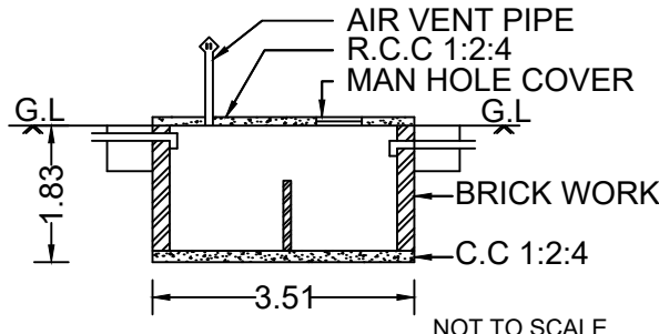
SEPTICTANK DETAILS
