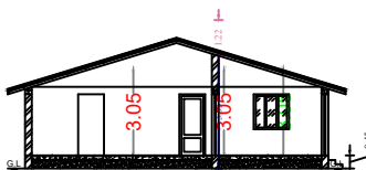
Section on-'RC'
