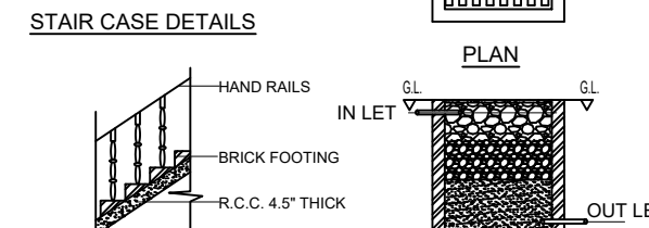
RAINWATER STORAGE PIT DETAILS
