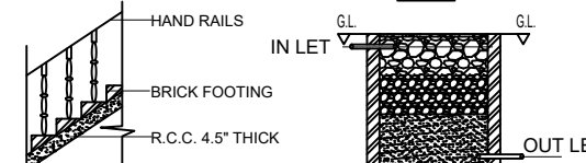
RAINWATER STORAGE PIT DETAILS
