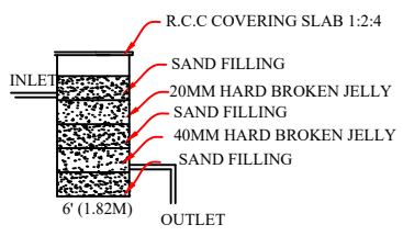
RAIN WATER HARVESTING SYSTEM
