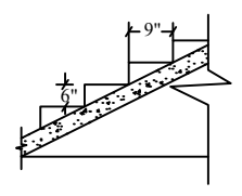
STAIR CASE DETAILS
