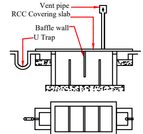
SEPTIC TANK
