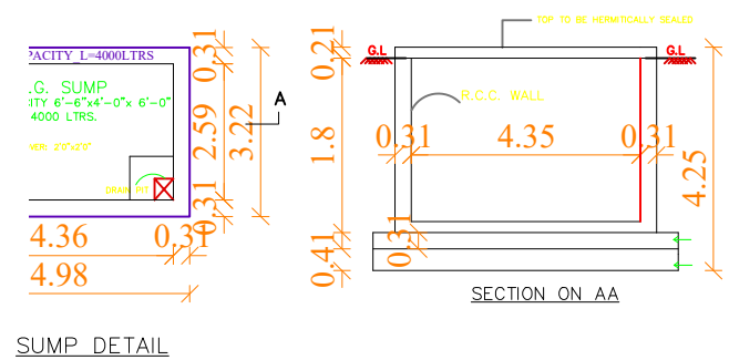
SUMP DETAIL
