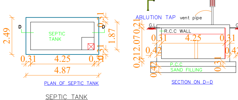
SEPTIC TANK
