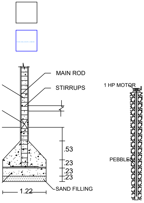
BORE WELL
